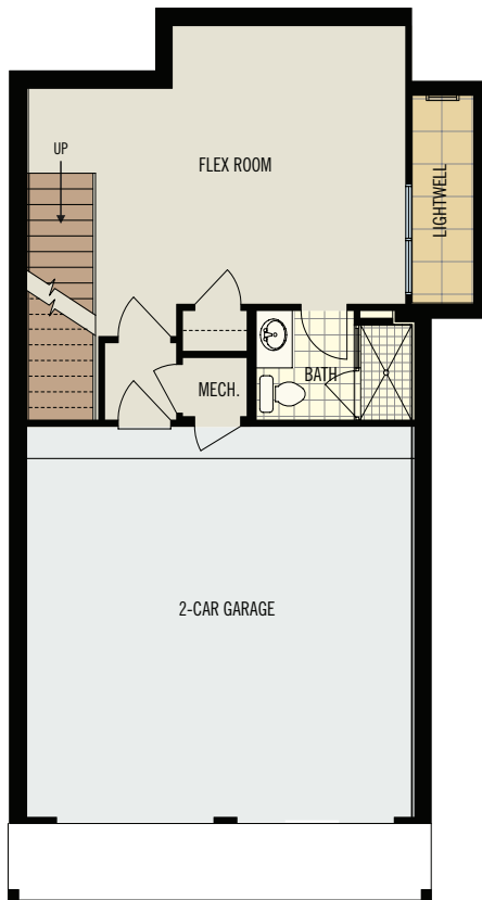
1st level (370 heated sq. ft.)
